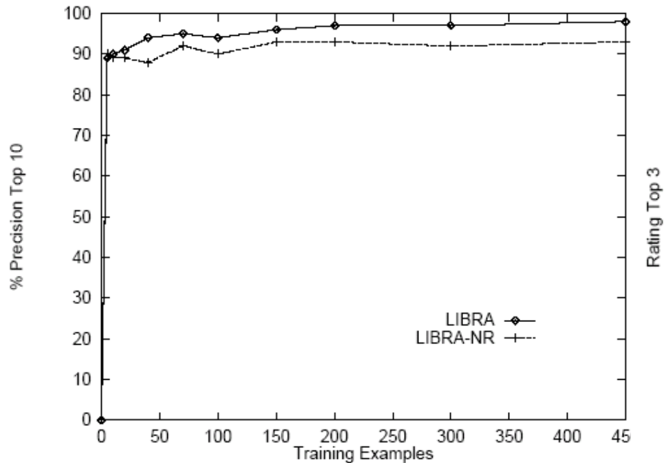
Figure 2: MYST Precision at Top 10
