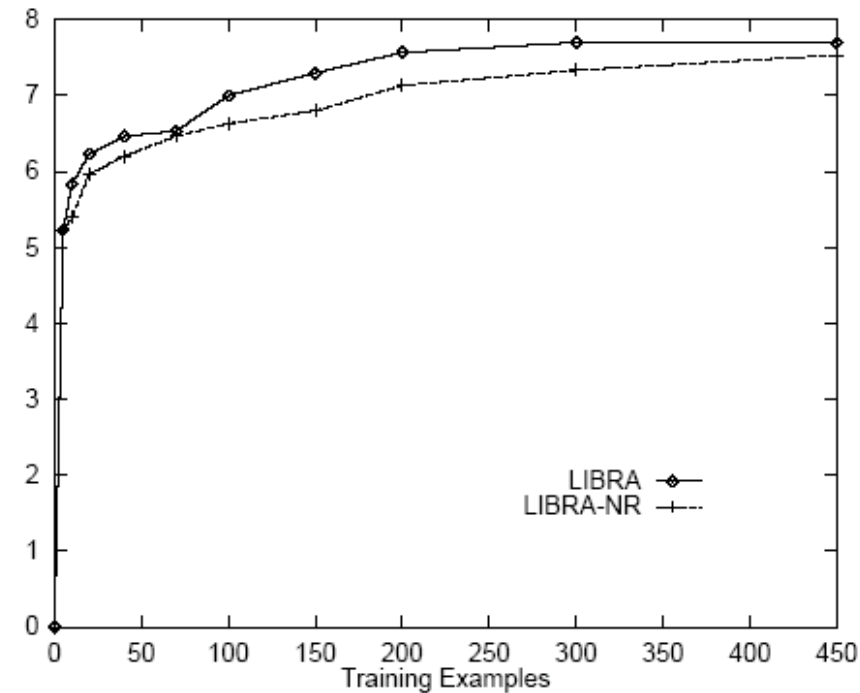
Figure 3: SF Average Rating of Top 3
