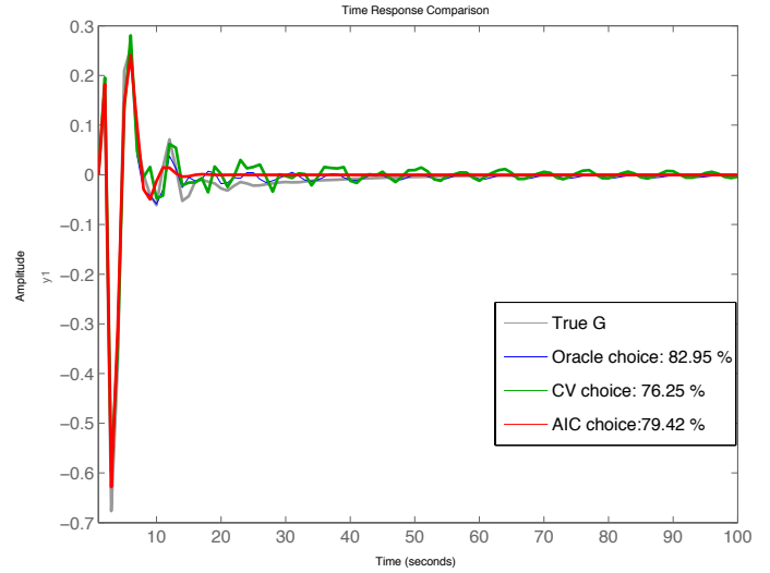
Fig. 9. The true impulse response of G compared to state space models of different orders. The figures refer to the “fit”, i.e. how much (in %) of the impulse response variation is reproduced by the model. 100% thus means a perfect fit.
