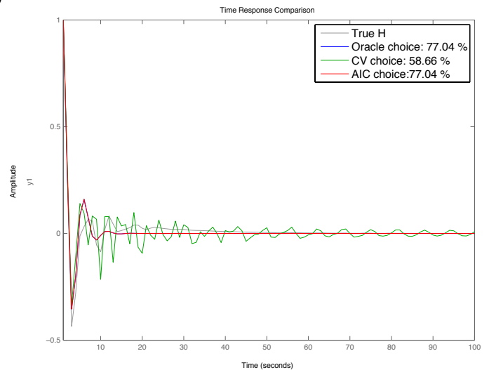
Fig. 10. The true impulse response of H compared to various models.
